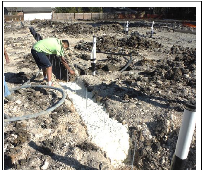
Suspended Plumbing with light-weight material covering plumbing prior to the slab pour and slab lift
