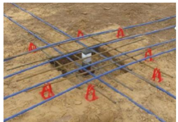
Detail of capital reinforcement
